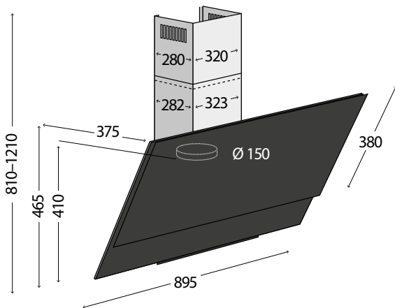
OPK4690, OPK4590bc
