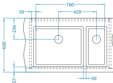
QUADRIX 10+50-FS
